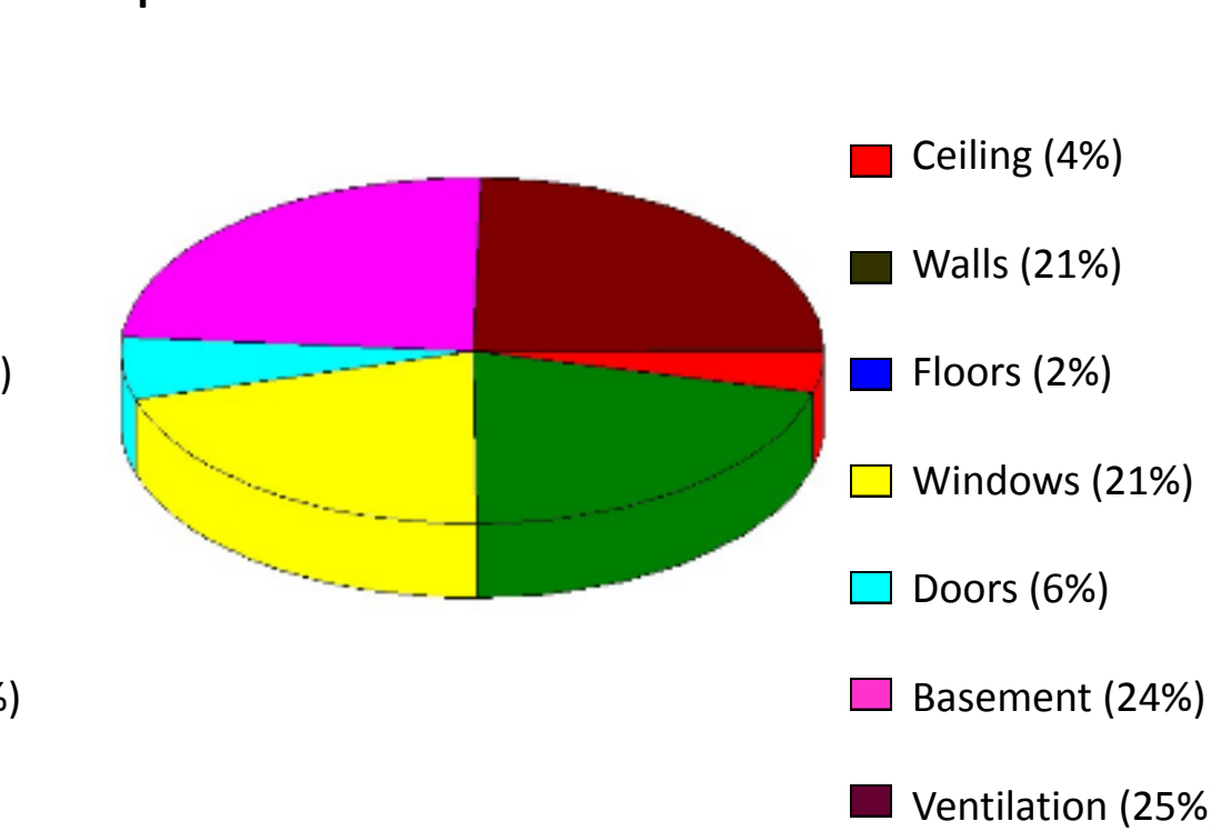
Components of Annual Heat Loss
