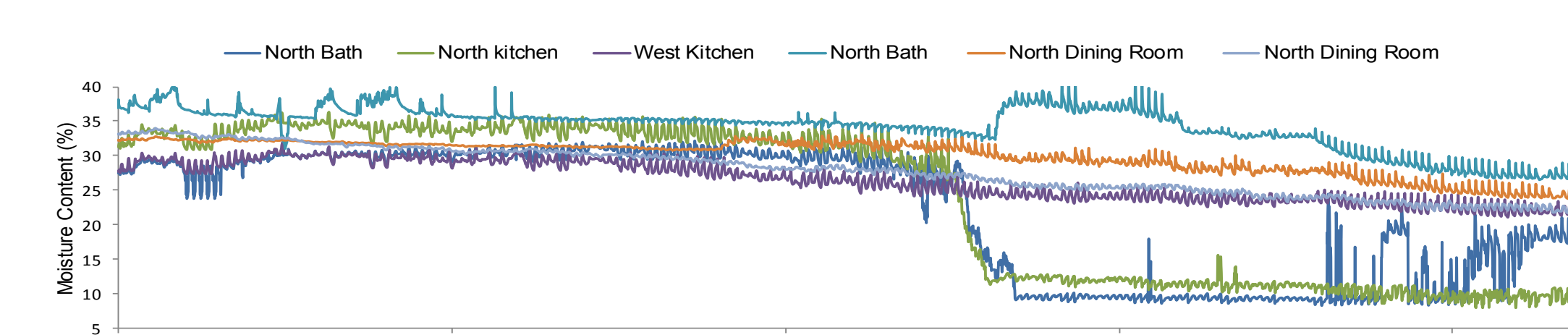
Hourly Moisture Content on Various Elevations
