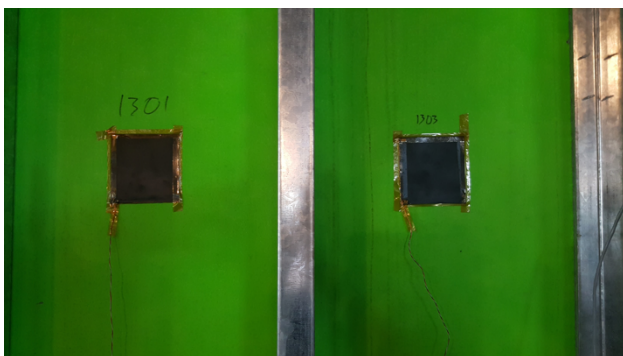
Figure 4. Interior Heat Flux Sensor Installation
