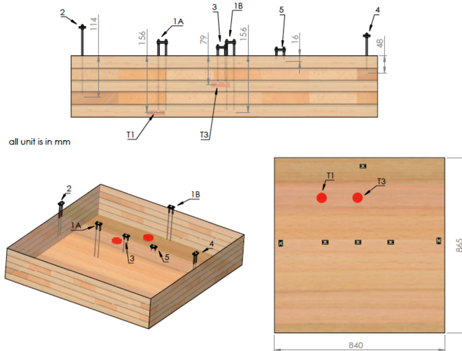
Figure 2: Probe Locations and Orientation
