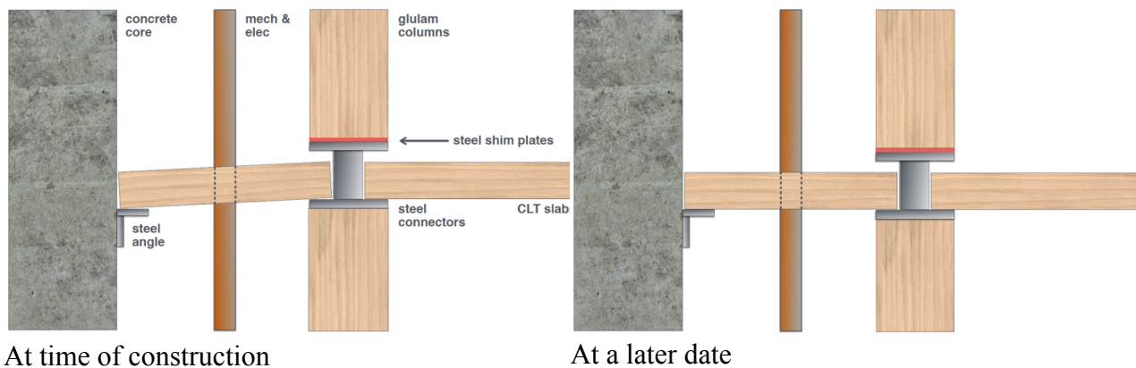
Figure 17: Setting Compensation in Structure Design (Acton, 2016)
