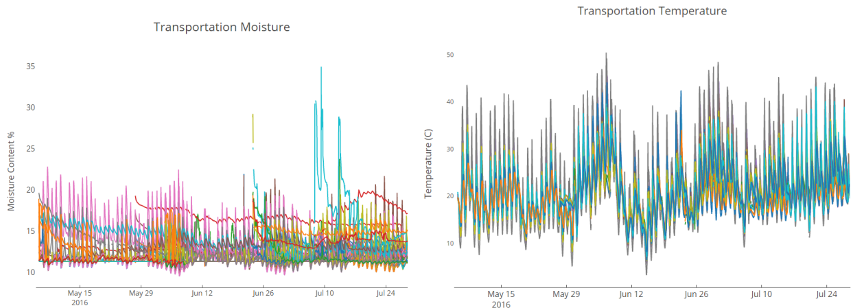
Figure 8: Transportation Moisture and Temperature Data
