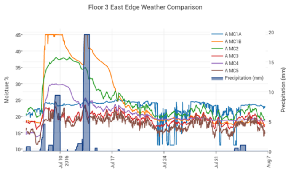
Figure 14: CLT Moisture Performance After Exposed Precipitation Event
