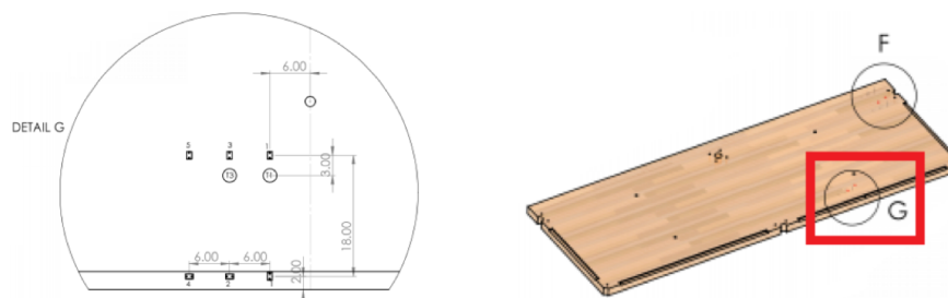
Figure 13: Plywood Spline Moisture Probe Location
