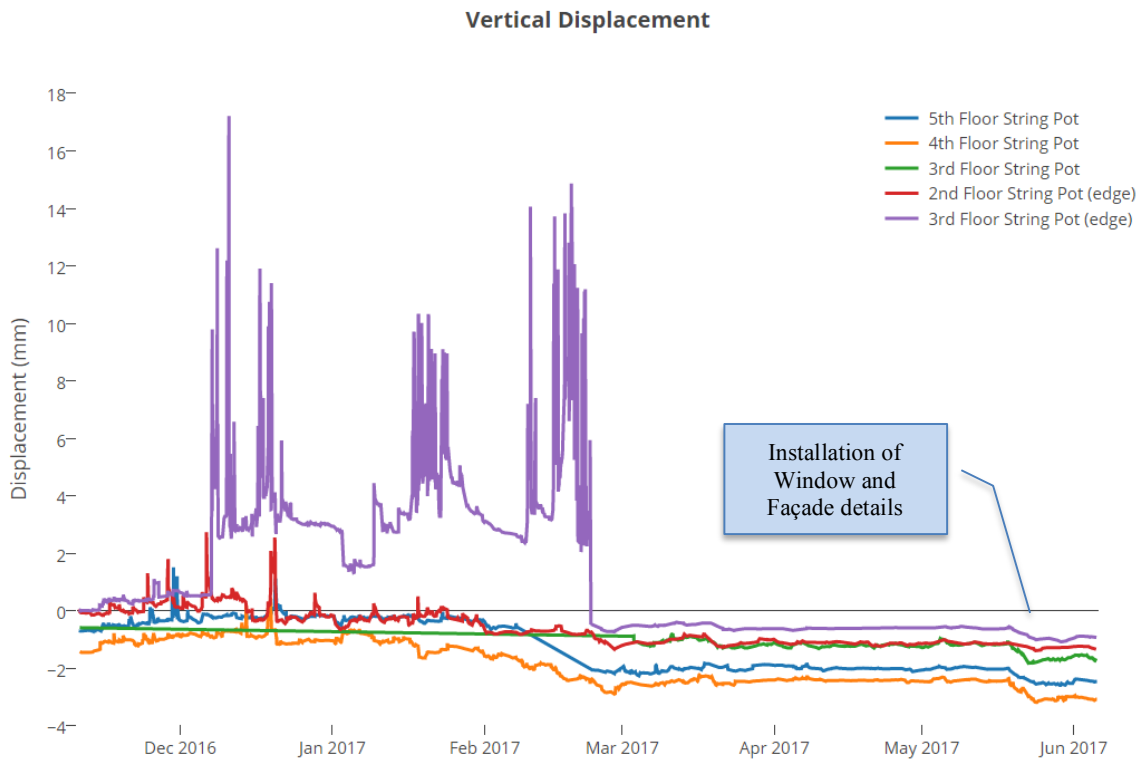
Figure 20: Vertical Displacement Sensor Data
