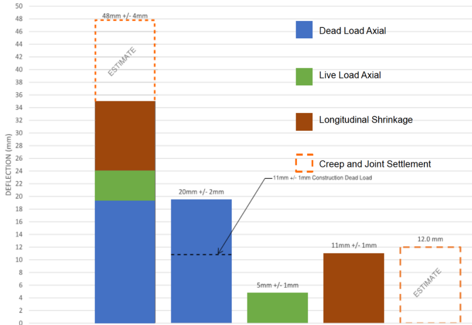
Figure 16: Column Shrinkage Estimation Calculated (Jackson, 2016)
