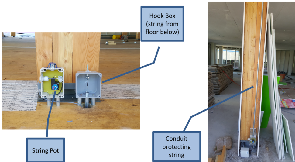
Figure 18: String Pot Units installed In Structure
