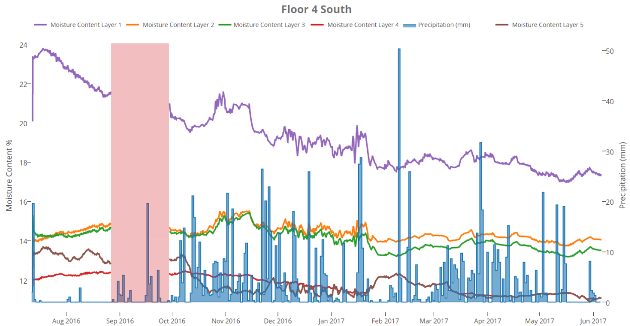
Figure 15: Year Long CLT Moisture Performance
