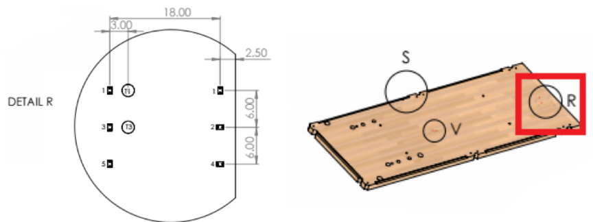
Figure 12: Edge Panel Moisture Probe Locations
