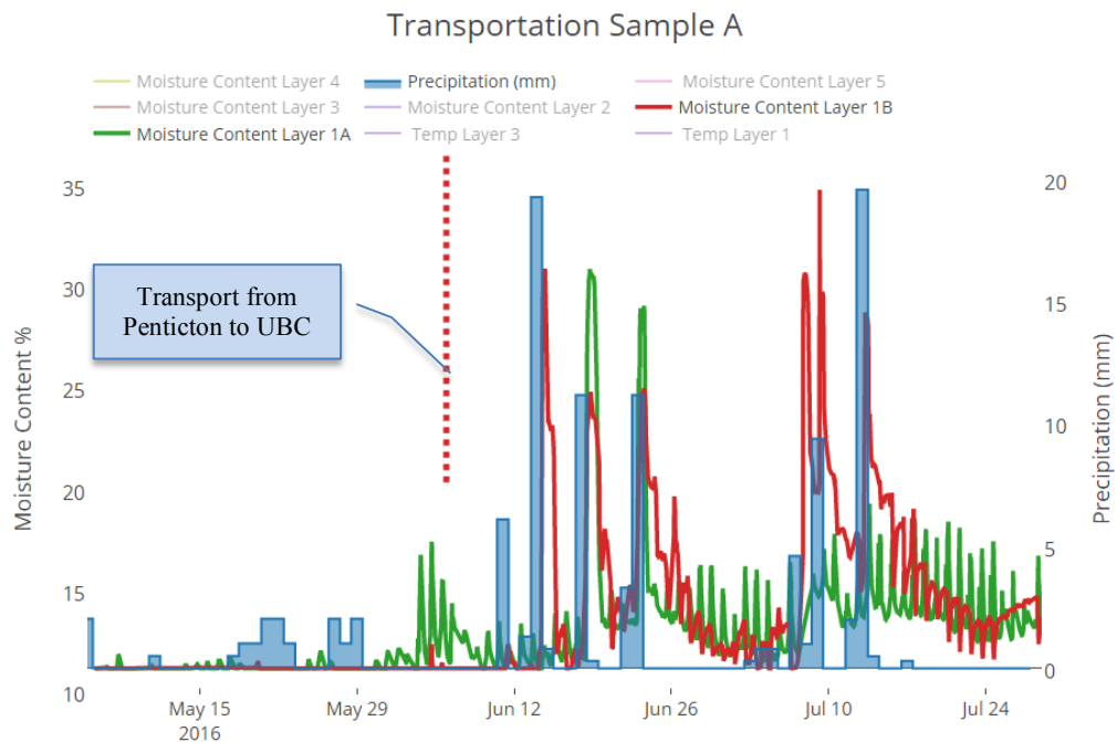
Figure 9: Analysis of Sample A during Transport
