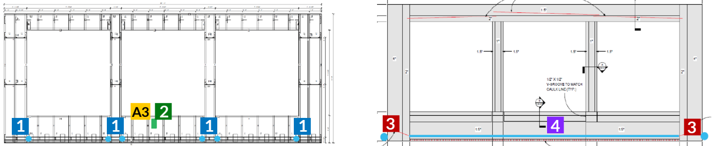
Figure 1: Proposed Sensor Locations in Panel System.
